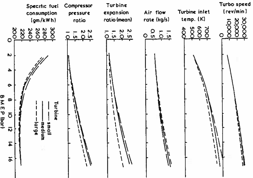
Figure 10.9 The effect of small turbine area change on engine performance at constant speed
