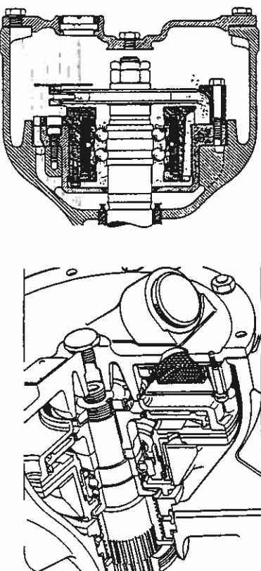
Figure 2.22 Oil disc pump lubrication (Brown Boveri and Napier)
