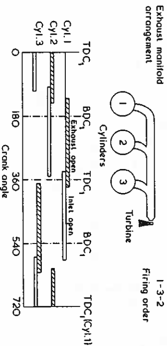
Figure 7.8 Pulse system: three-cylinder four-stroke engine with automotive-type valve timing
