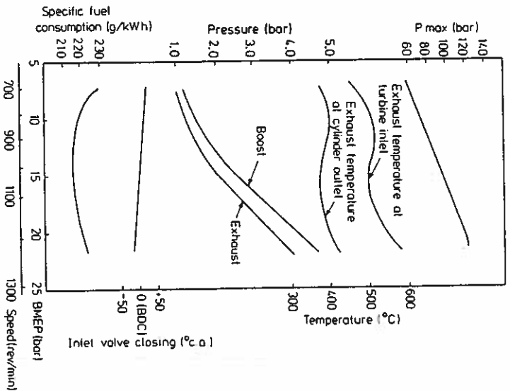
Figure 11.7 Propeller law performance with the Miller system and two-stage turbocharging [7]
