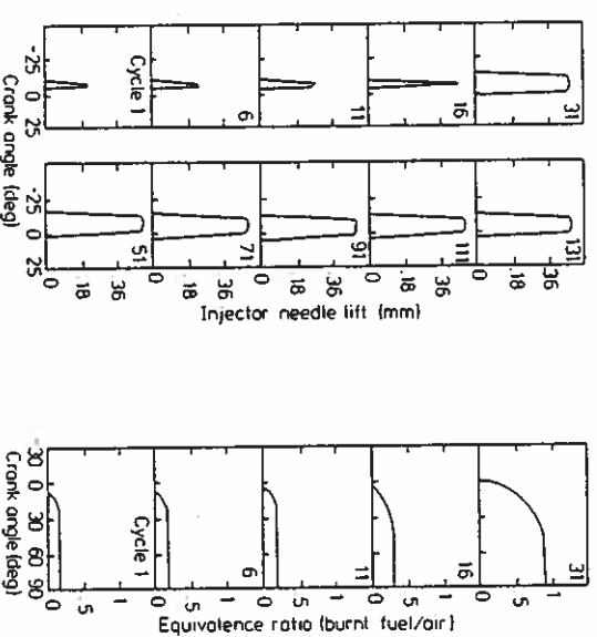
Figure 12.2 Detailed engine performance parameters during the load change shown in figure 12.1
