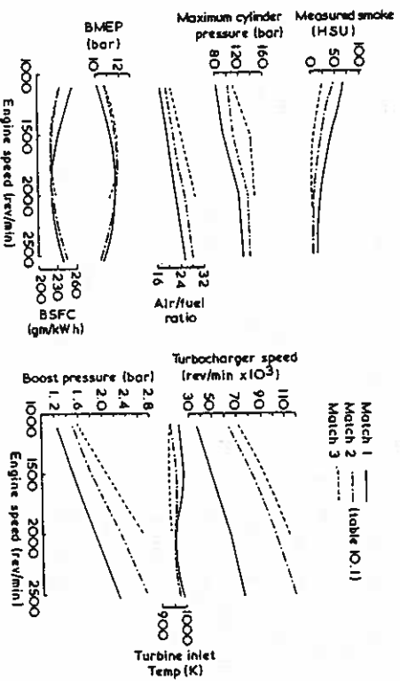
Figure 10.24 The effect of turbine match on engine performance with no change in fuelling [6]
