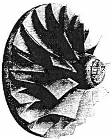
Figure 2.34 Impeller with splitter vanes (Holset)
