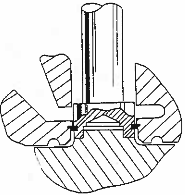
A single piston ring locates in a stepped bore bearing housing.
