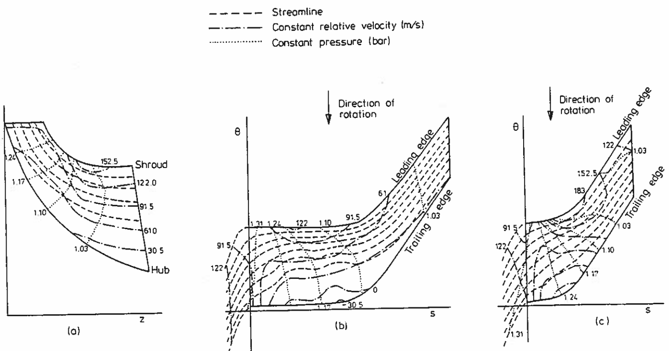
Figure 4.28 (a) Flow pattern in meridional hub-to-shroud plane; (b) flow pattern in blade-to-blade plane on hub surface; (c) flow pattern in blade-to-blade plane at shroud surface [19]
