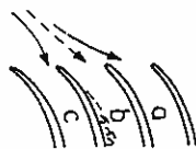
Figure 3.60 Rotating stall schematic
