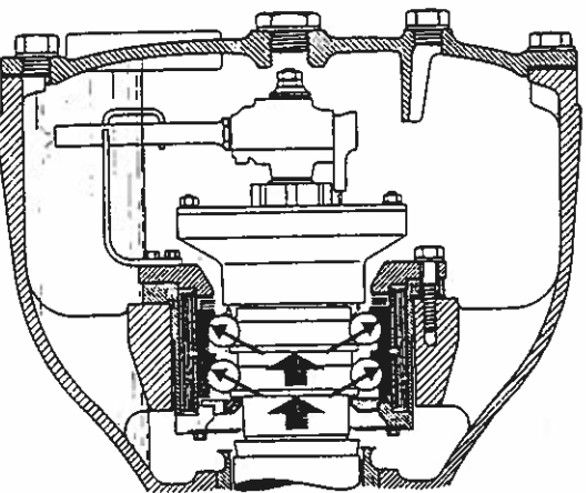
Figure 2.27 Rolling bearing with auxiliary plain thrust bearing (Brown Boveri)
