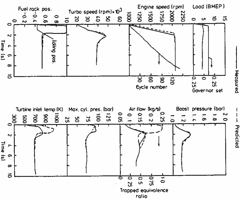
Figure 15.58 Measured and predicted response to an increase in demand speed [19]
