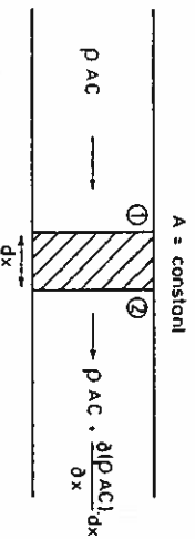
Figure 15.38 Mass flow rate into and out of a fluid element in a pipe (constant cross-sectional area)
