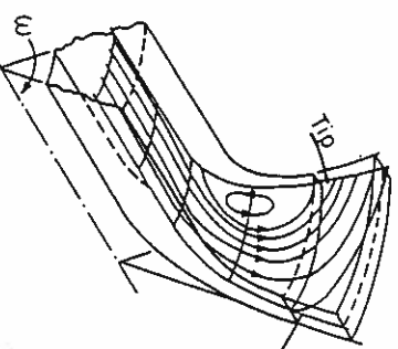
Figure 3.48 Relative streamlines in 'blade-to-blade' solution
