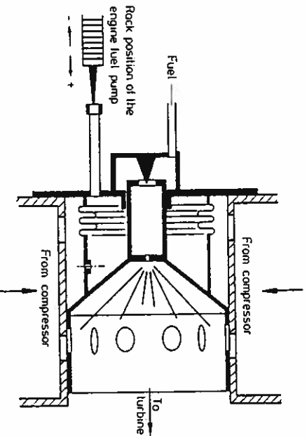
Figure 11.34 Hyperbar auxiliary combustion chamber schematic [27]
