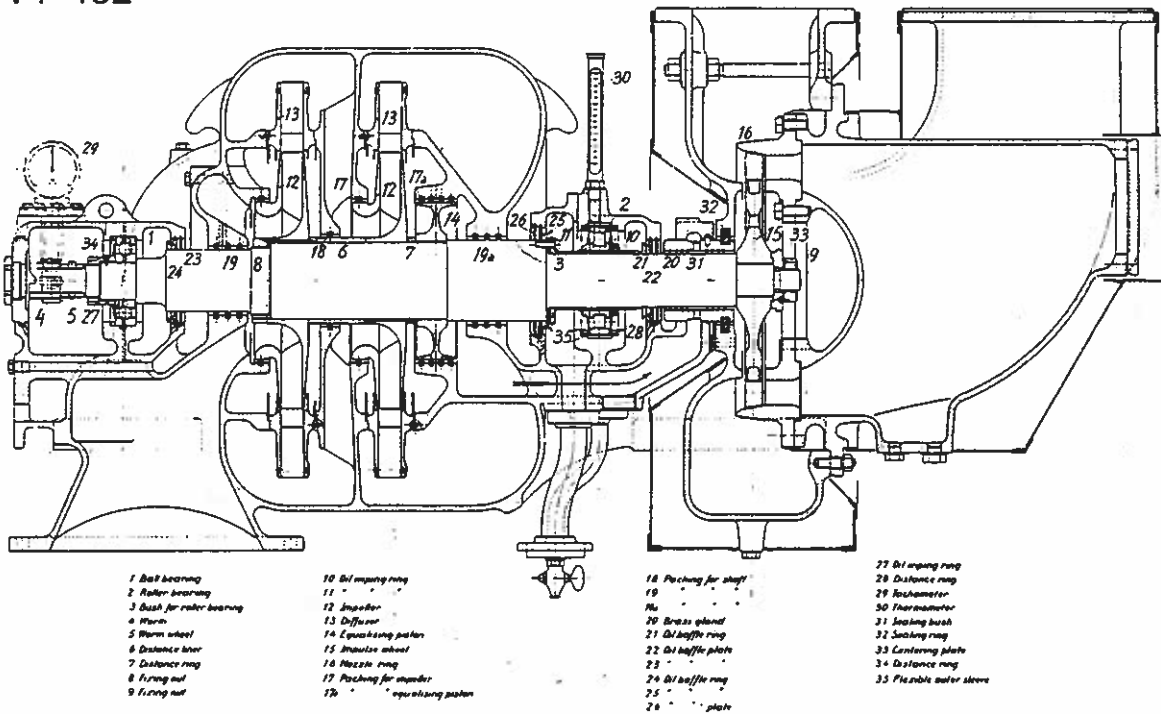
Figure 2.20 One inboard and one outboard mounted bearing
