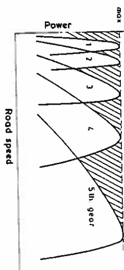
Figure 10.20 Power/speed envelope for a five-speed gearbox truck
