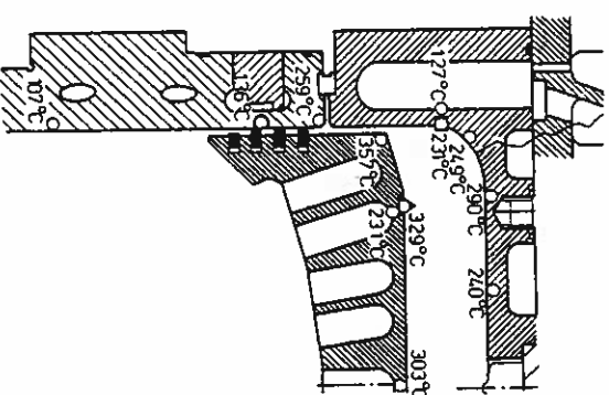
Figure 11.12 Drilled liner cooling passages on a MAN two-stroke engine
