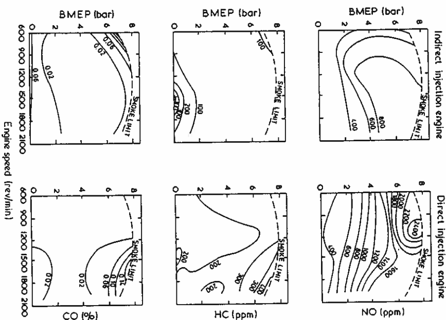
Figure 14.8 Typical exhaust emission maps from direct and indirect (swirl chamber) injection engines [7]
