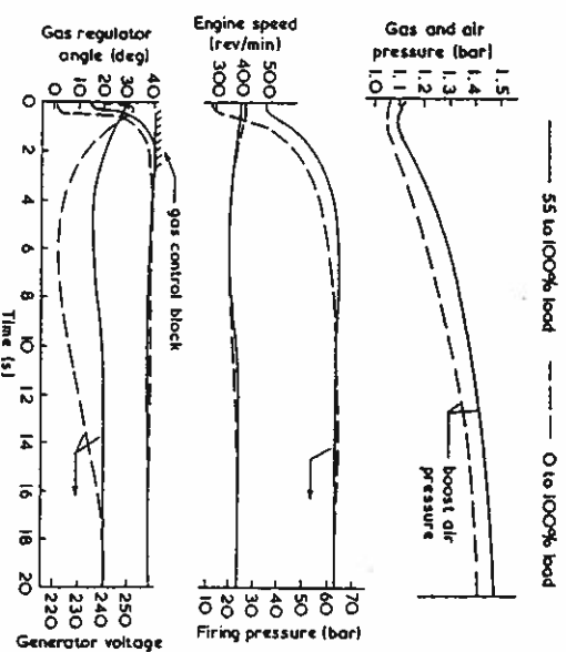
Figure 12.5 Natural gas engine generator response to load changes [2]
