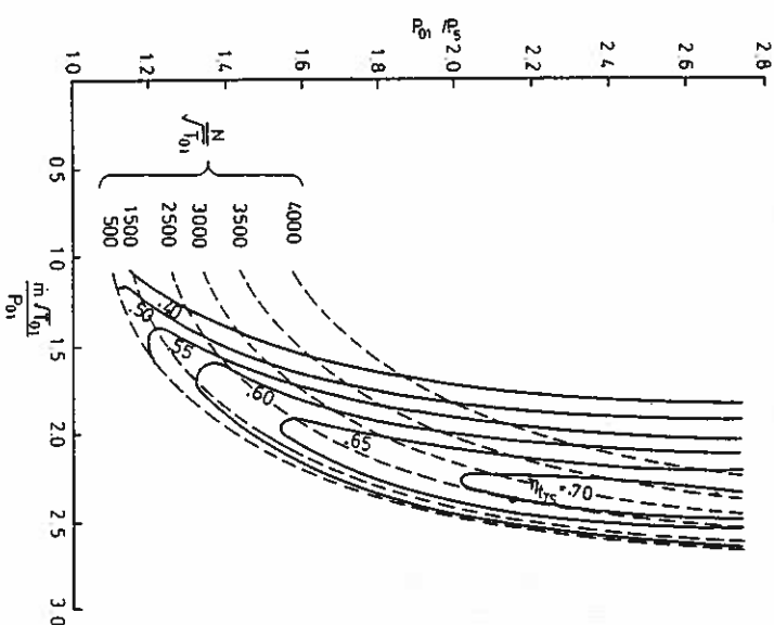
Figure 4.33 Typical turbine characteristic (Holzer Ltd)
