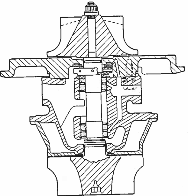
Figure 2.26 Floating bush plain bearing mounting (Garrett)
