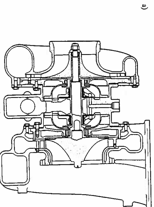
Figure 2.39 Small industrial turbochargers: (a) Napier,
