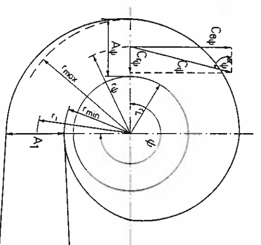
Figure 4.6 Volute-type turbine scroll
