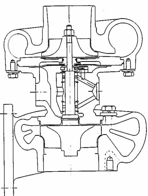
Figure 2.31 Holset H1B turbocharger
