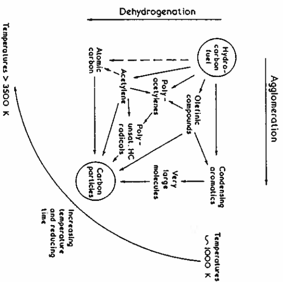
Figure 14.6 Simplified carbon formation scheme [5]
