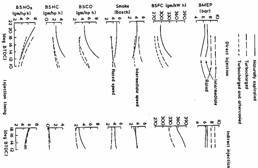
Figure 14.17 The effect of retarded timing on emissions and performance of turbocharged engines (13 mode cycle unless stated) [13]
