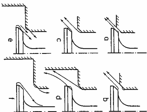
Figure 15.18 Flow pattern for inflow and outflow through a poppet valve
