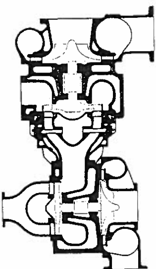
Figure 11.21 Cross-section of a Hispano Suiza two-stage turbocharging unit: left, the low-pressure stage; right, the high-pressure stage
