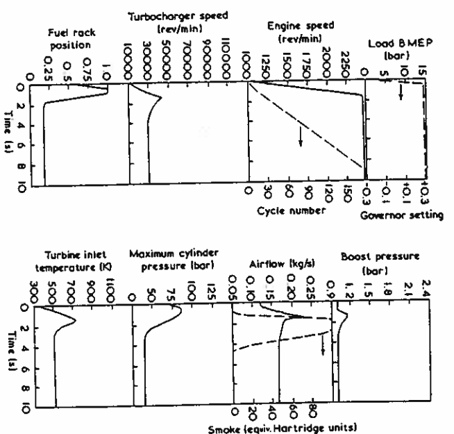
Figure 12.14 Free (no-load) acceleration of a truck engine
