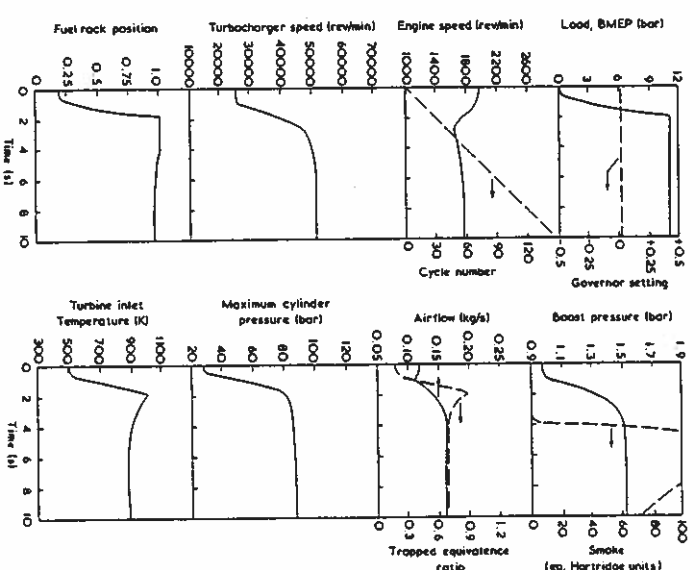
Figure 12.1 Engine response to a fast load application
