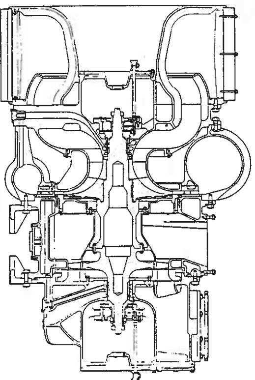
Figure 2.43 Sectional view of S610 (Napier)
