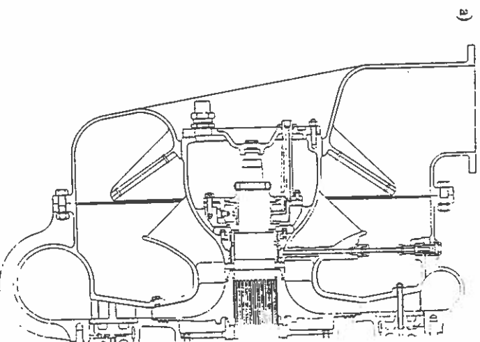
Figure 2.30 Silencers: (a) baffle (Napier)
