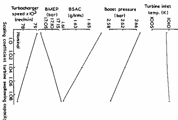
Figure 15.34 Effects of varying turbine area on engine performance
