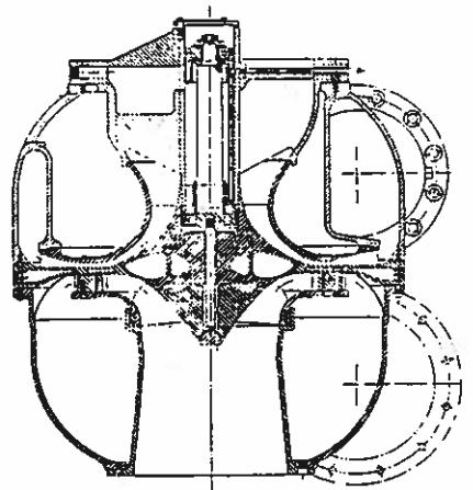
Figure 2.21 Outboard mounted bearings at one end (De Javal)
