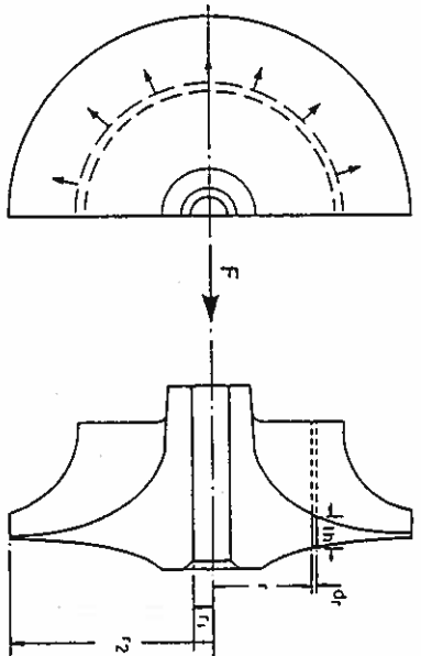
Figure 3.69 Estimation of 'bursting speed' coefficient
