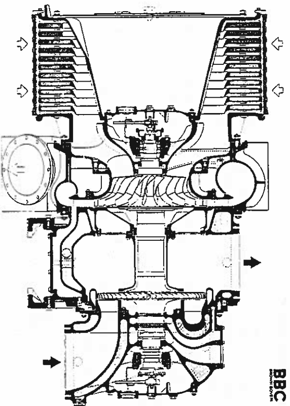
Figure 2.42 Sectional view of VTR 454 (Brown Boveri)
