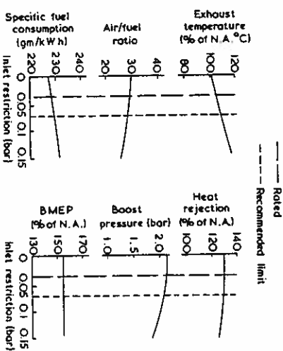
Figure 9.14 Influence of inlet restriction on engine performance [10]
