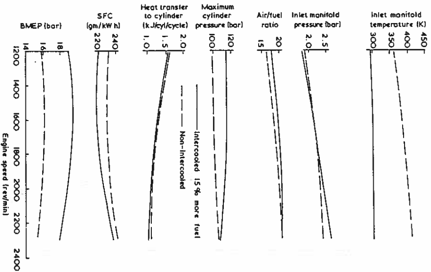
Figure 9.11 The effect of intercooling on engine performance (increased fuelling)
