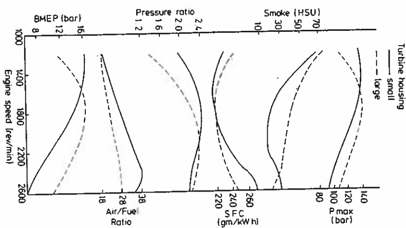
Figure 11.30 Engine performance with different turbine housings [24]
