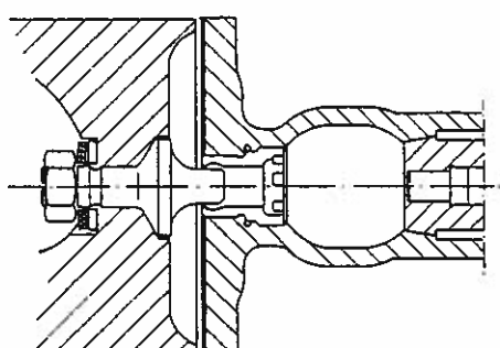
Figure 11.6 Arrangement of the variable geometry combustion chamber on the SEMT-Pielstick PA 4-185 engine
