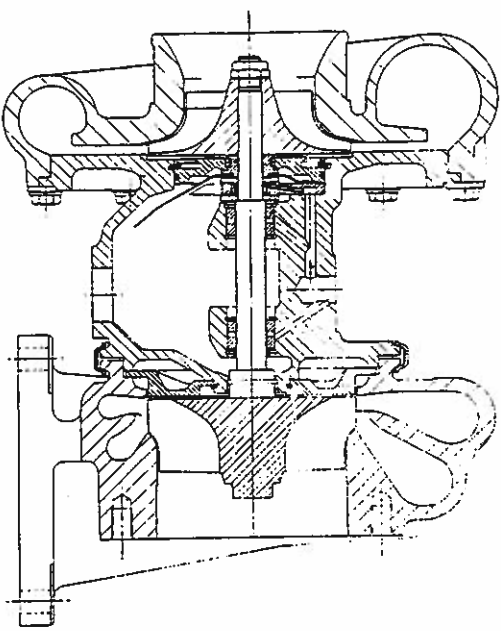
Figure 2.19 Inboard mounted bearings (Holset)
