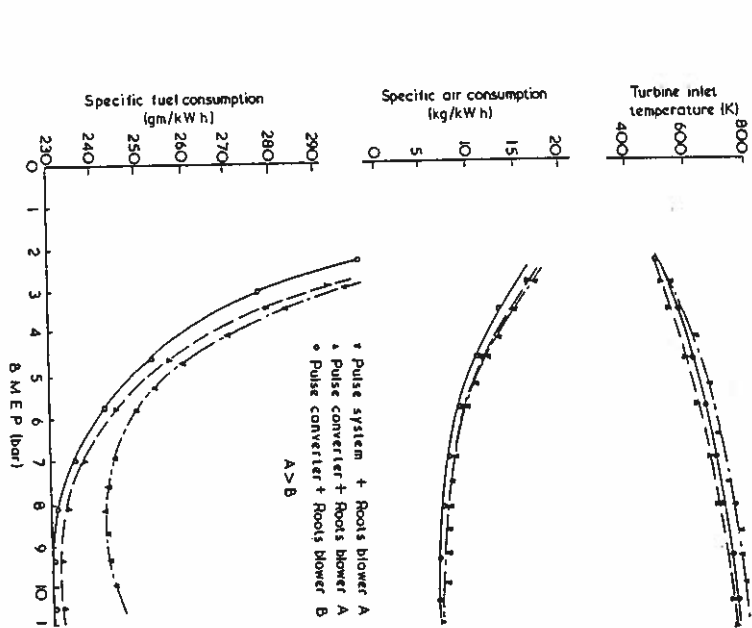
Figure 8.7 Comparison of performance at 1500 rev/min of pulse and pulse converter systems (four-cylinder two-stroke engine)
