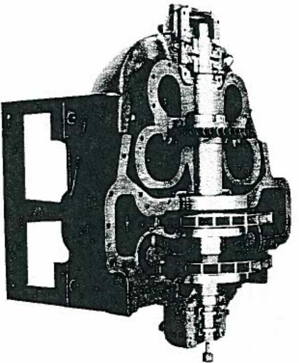
Figure 2.15 One of the first Brown Boveri turbochargers
