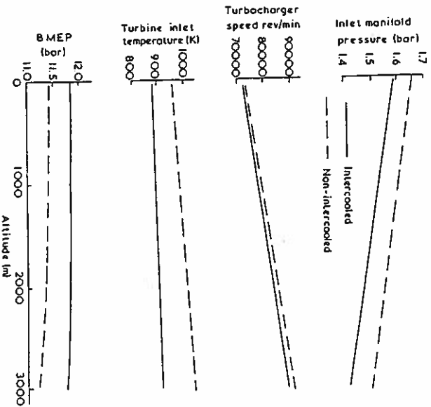
Figure 10.36 The effect of altitude on truck engine performance
