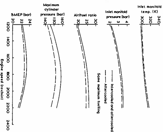
Figure 9.12 The effect of interstage cooling on two-stage turbocharged engine performance
