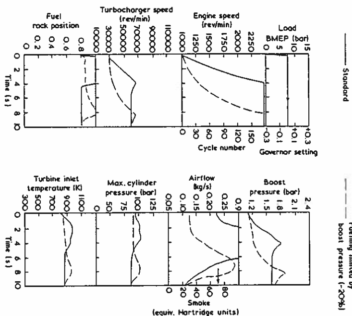
Figure 12.15 The effect of boost control of fuelling on acceleration under load
