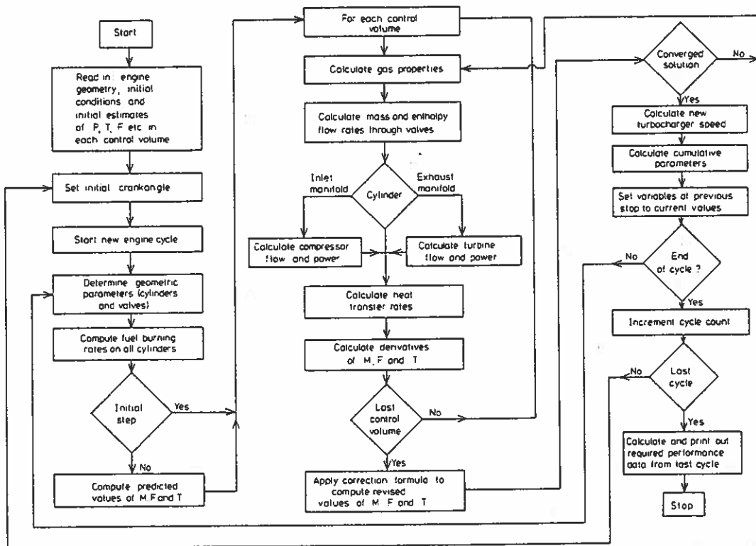
Figure 15.29 Flow diagram for 'filling and emptying' model
