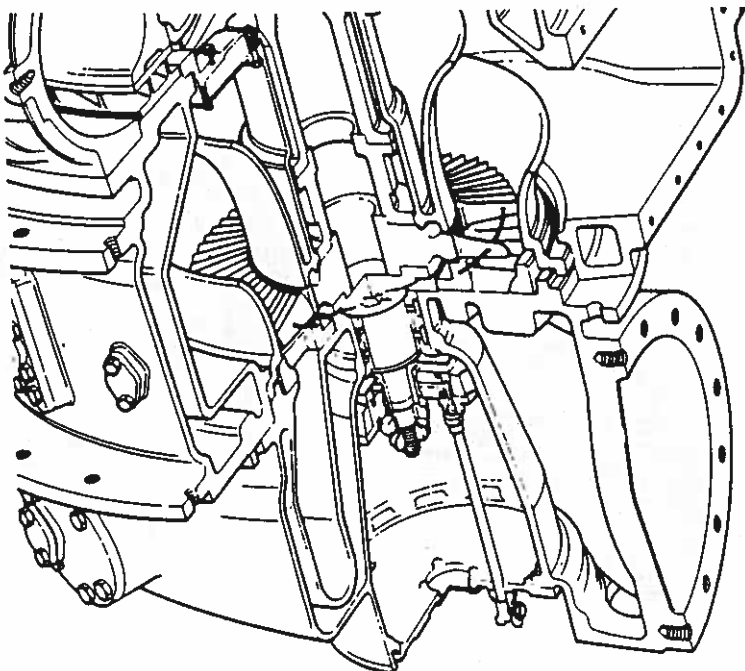
Figure 2.3 Axial flow turbine (Napier)
