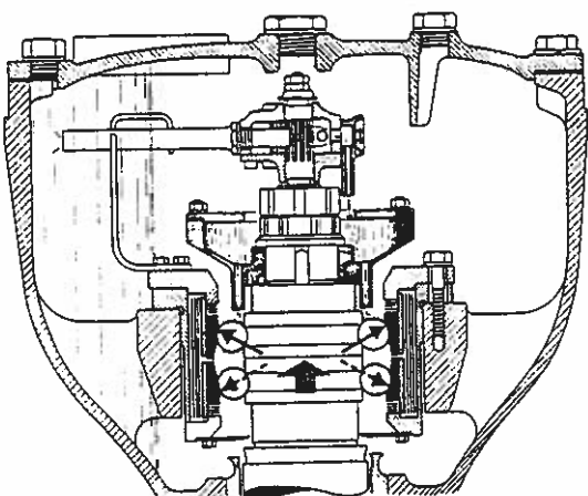
Figure 2.23 Gear pump lubrication (Brown Boveri)
