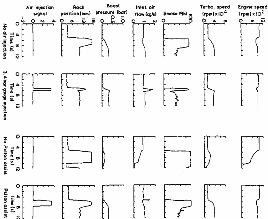
Figure 12.22 Comparison of air injection and Pelton wheel oil assistance on response to a step load application [5]
