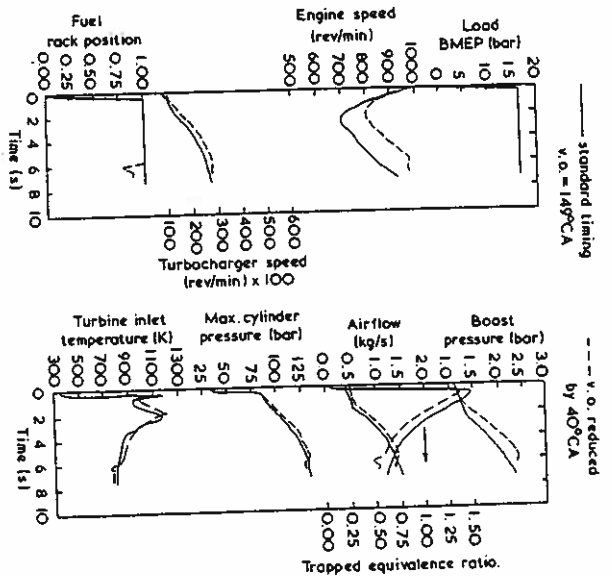
Figure 12.13 Effect of valve overlap on load acceptance of a medium-speed turbocharged diesel engine
