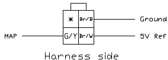
Connector EM-37
