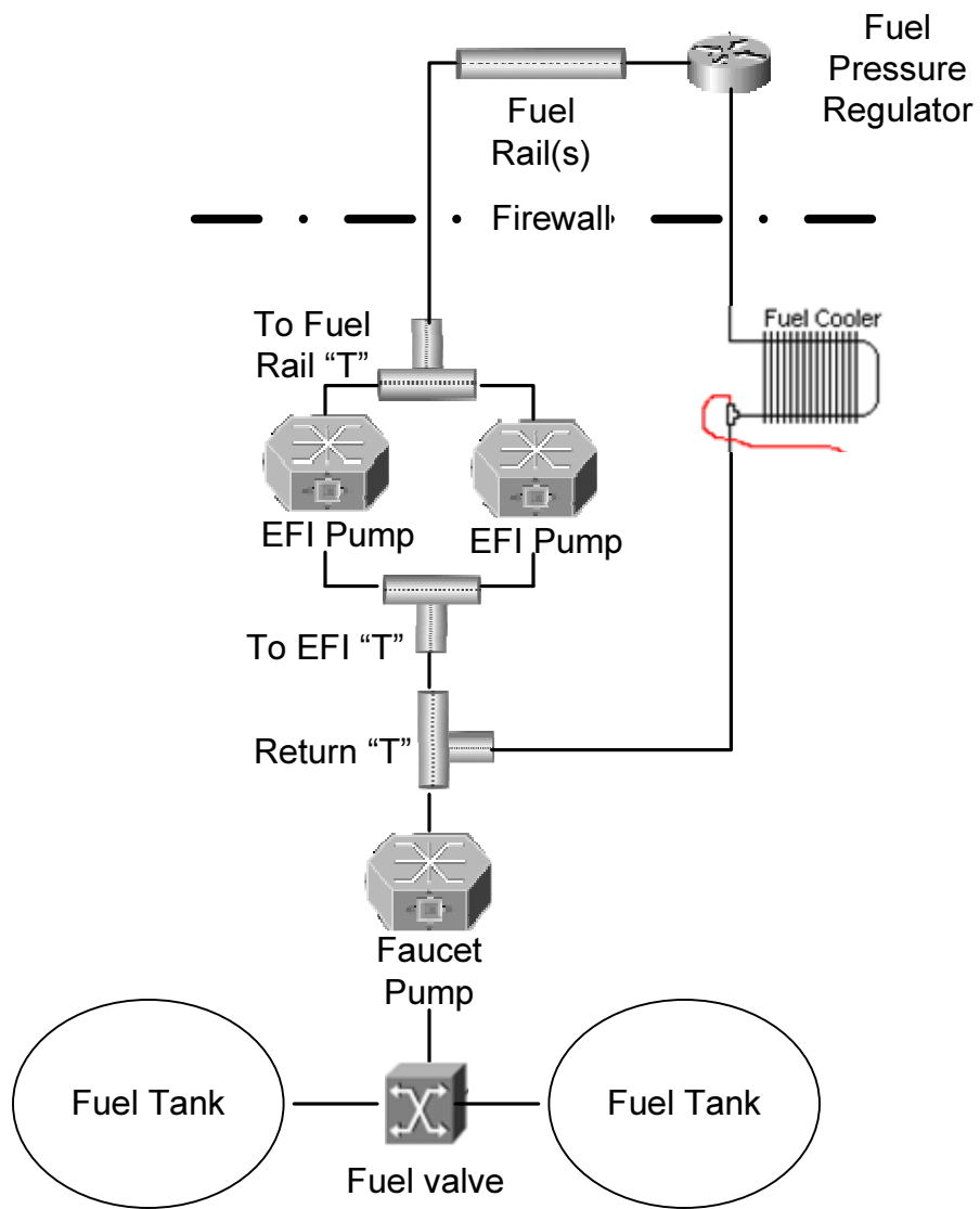
Semi-Returnless Fuel system
