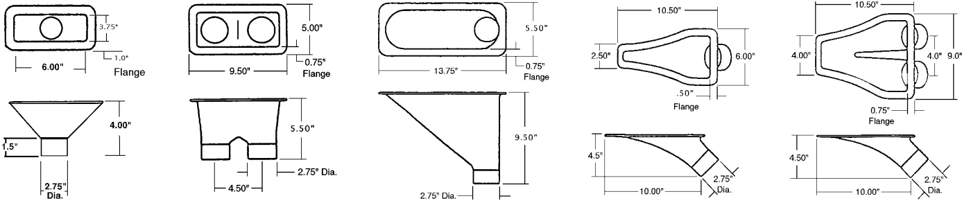
Headlight Mount Air Inlet Part No. 3623
