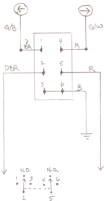
GENERIC DPDT SWITCH WIRING
