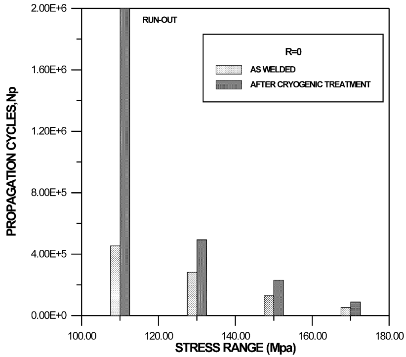
Fig. 6. Comparing crack propagation cycles of treated and non-treated joints.
