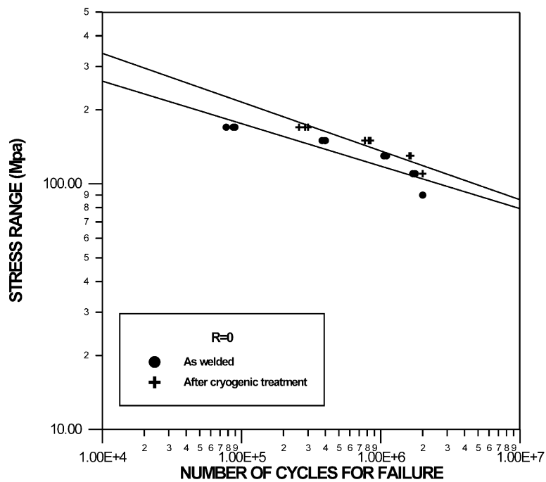
Fig. 7. S-N curves.
