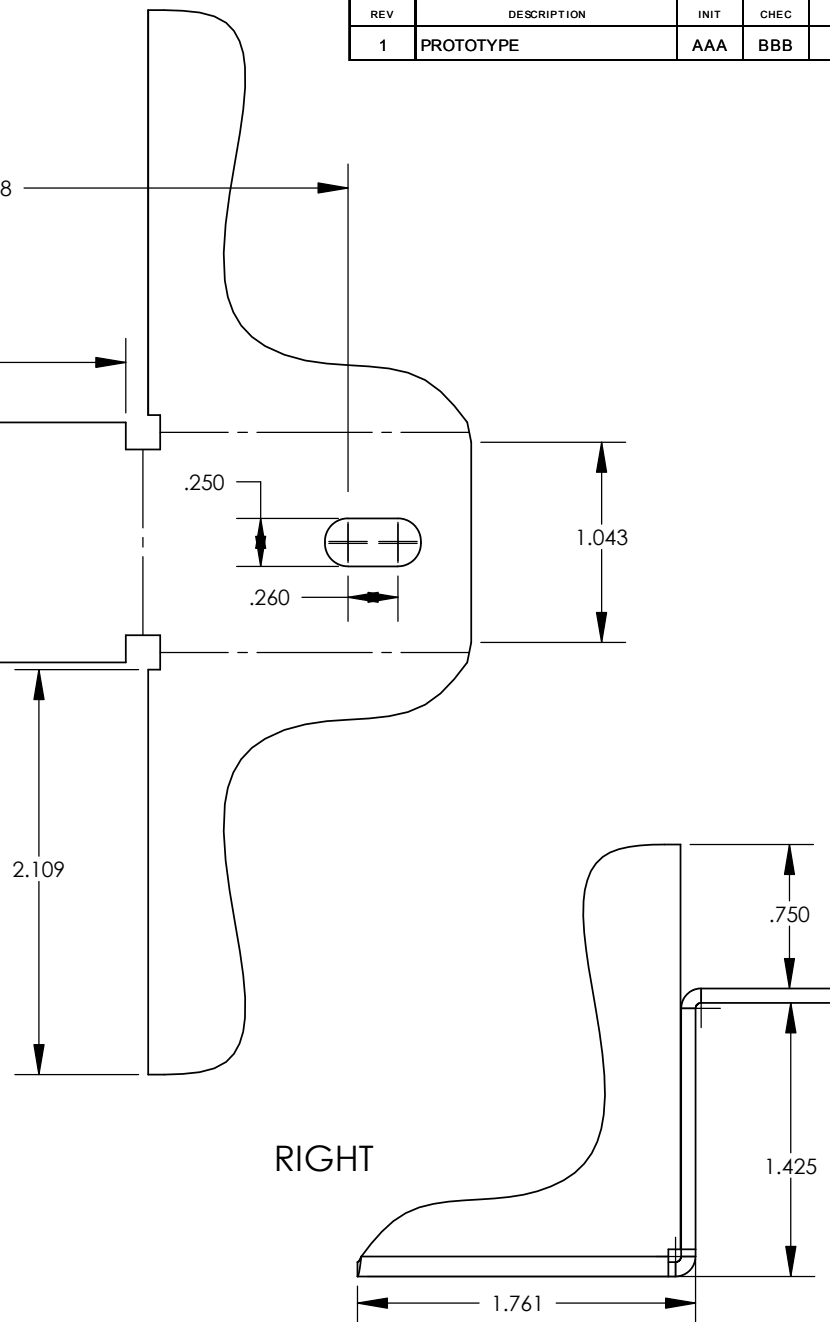
FLAT PATTERN
