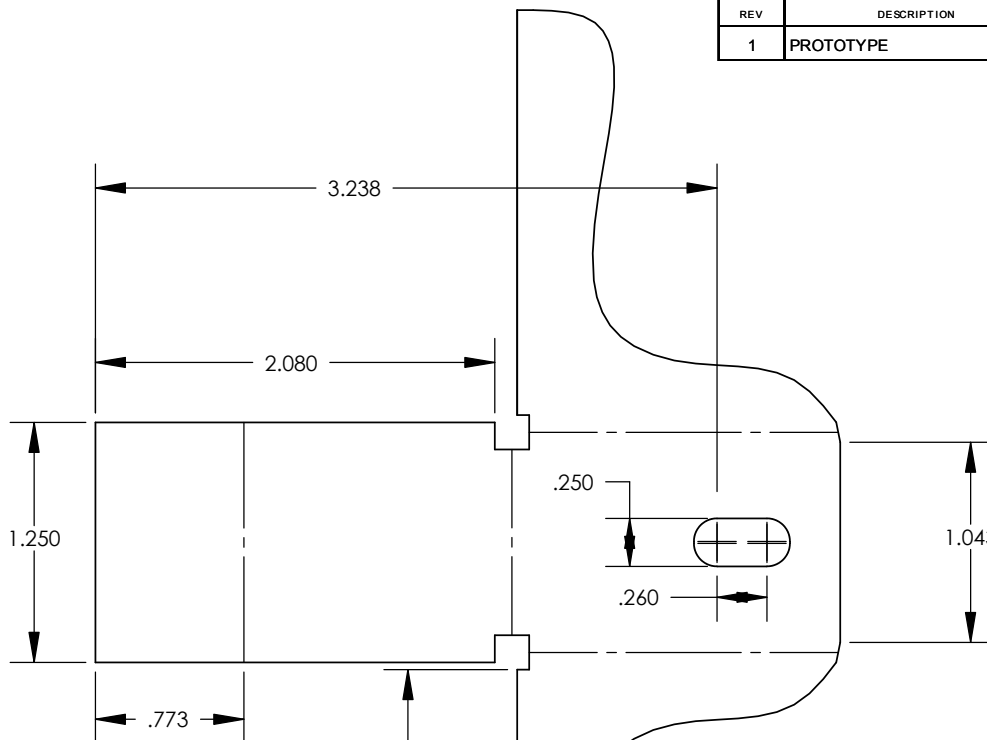
FLAT PATTERN
