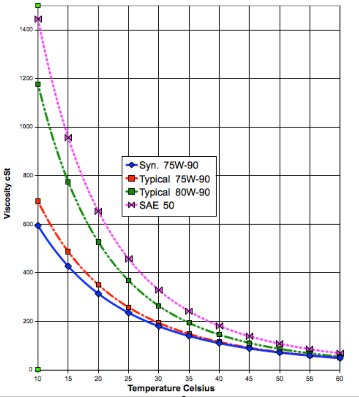
Viscosity Curve
