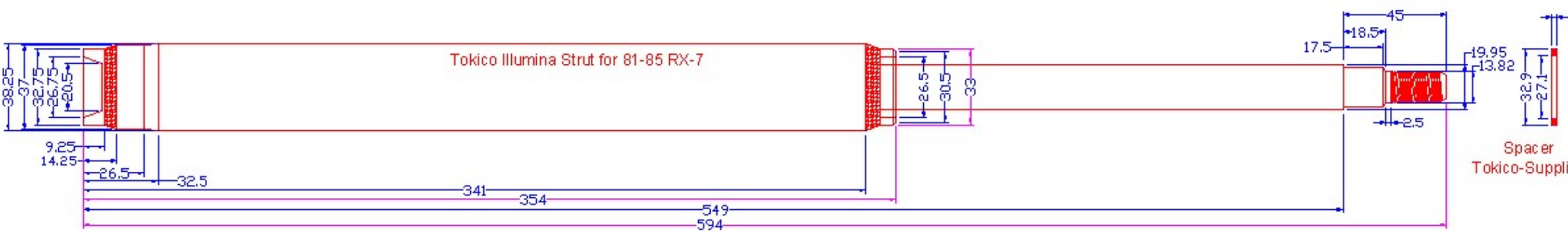
Threaded Section Full Round; Hex Key Indent @ End
